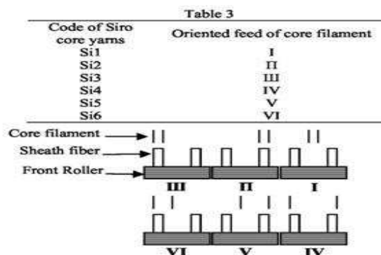
Fig1- different states of feed of core filament on siro core yarns
