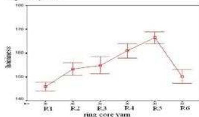
Fig4- effect of filament pre-tension on hairiness of ring core yarns
